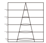
Illuminance Characteristics
