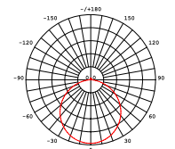
Illuminance Characteristics
